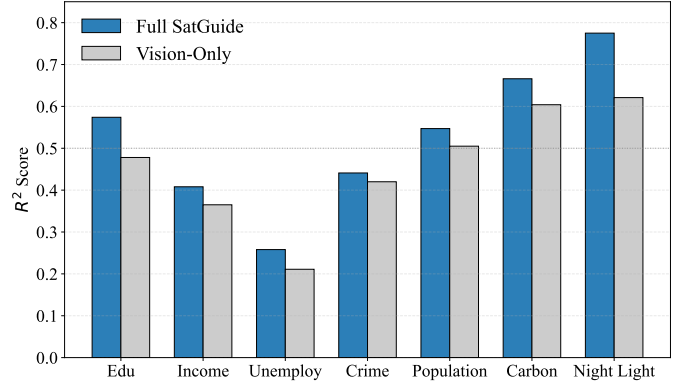
Fig. 9. Performance comparison between full SatGuide (with POI anchor) and its vision-only variant (without POI) across seven prediction tasks. The vision-only branch maintains competitive prediction accuracy even in the absence of POI data, demonstrating the robustness of our visual learning framework for POI-sparse regions.
