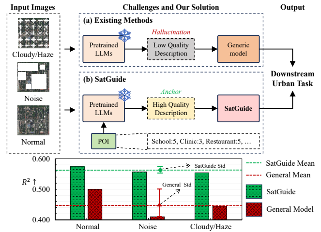
Fig. 1. The illustration of challenges and our solution. Left includes real-world satellite images of different qualities. Middle-upper explains the reason of robustness issue. Middle-lower shows our enhancement towards the robustness. Histogram demonstrates that SatGuide alleviate this issue effectively.
